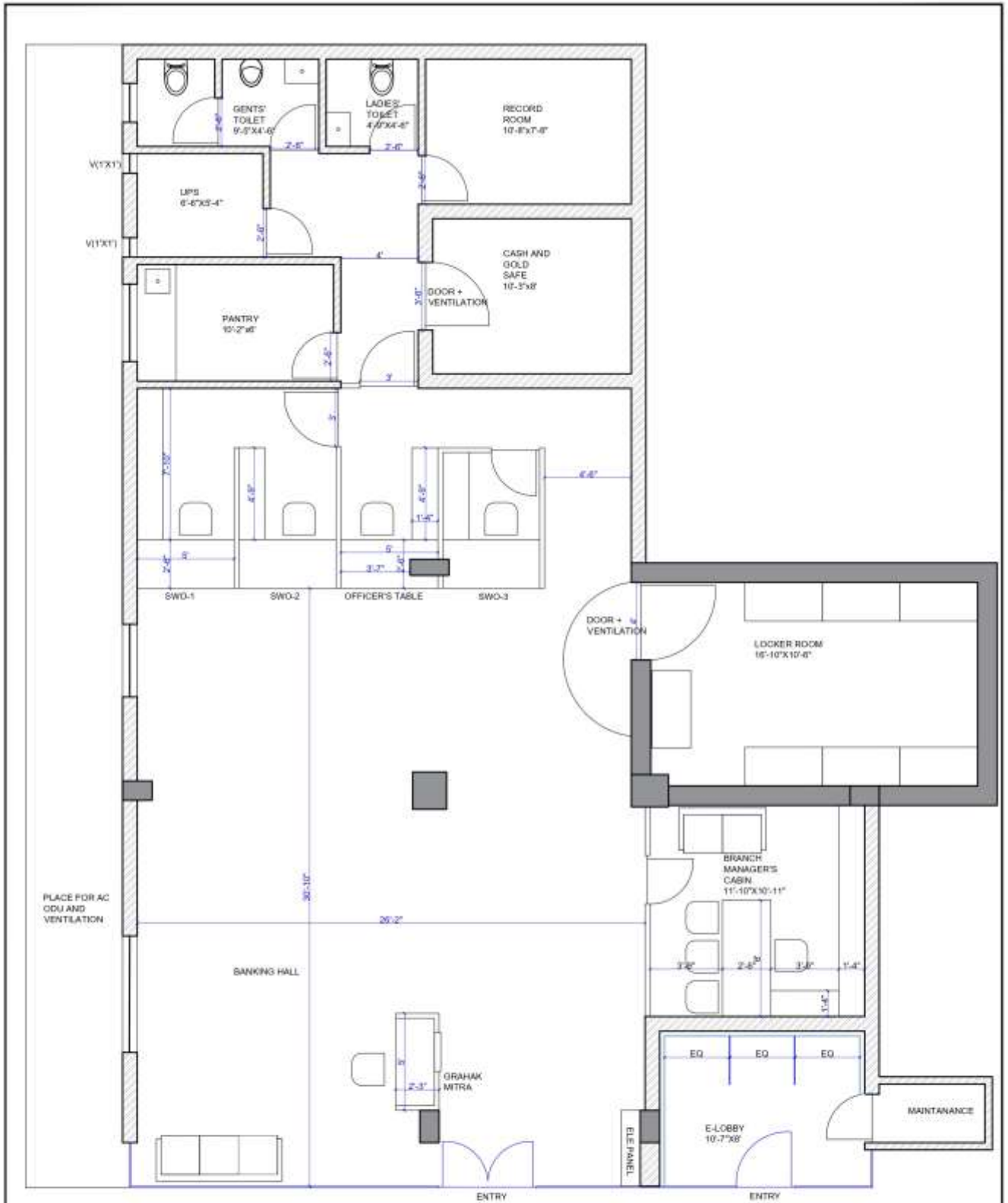
FURNITURE LAYOUT OPTION -1
